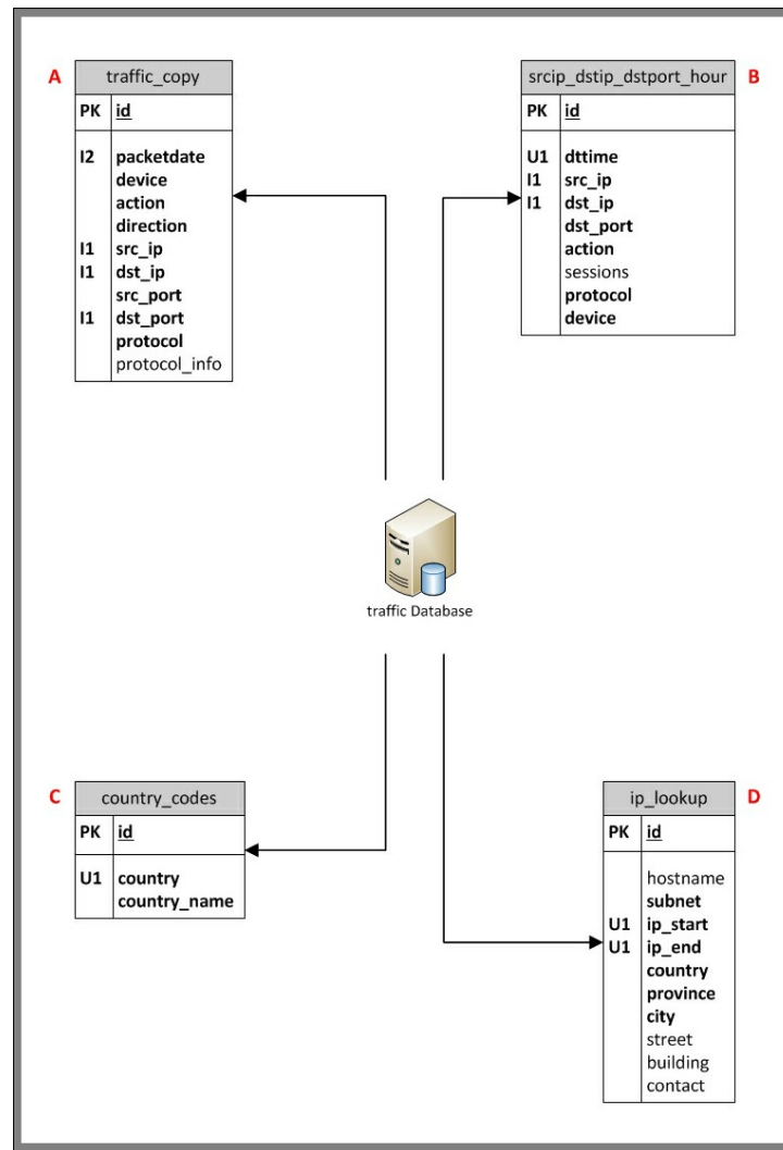
Figure 3.2: Database layout
