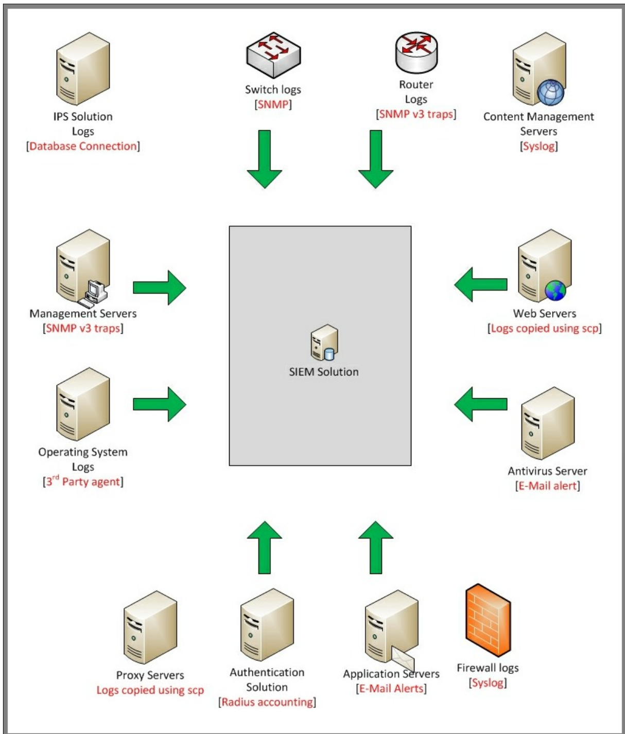
Figure 2.2: SIEM Architecture
